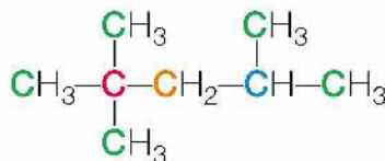
2,2,4-trimetylopentan
