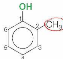
2-metylobenzenol
