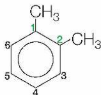
1,2-dimetylobenzen
