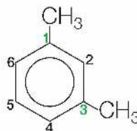
1,3-dimetylobenzen
