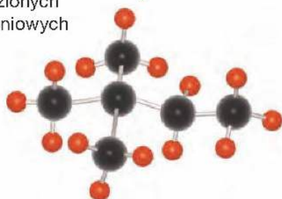
2,2-dimetylobutan
