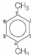
1,4-dimetylobenzen
